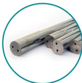
双直孔棒 Rods with Two Straight Coolant Holes
